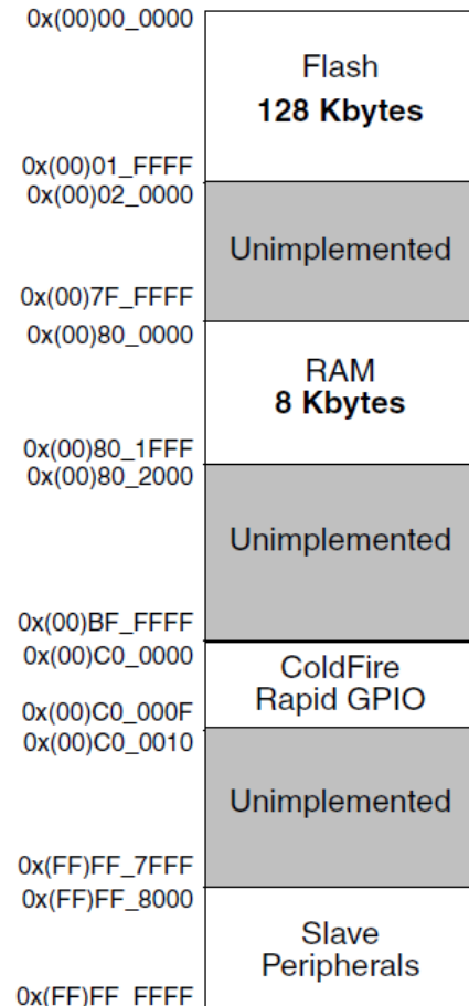
ColdFire MCF51QE128
